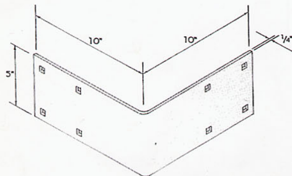
Corner Plate (No Tabs) 6H406
