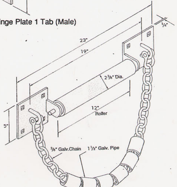
Pile Chain & Roller Kit 9H419
