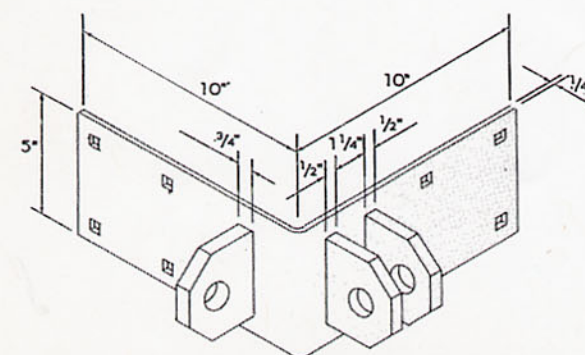
Corner T-Hinge PL 3 Tab (Male Female) 6H409
