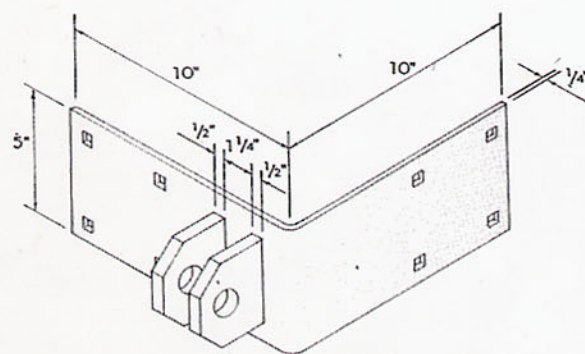
Corner Hinge Plate 2 Tab (Female) 6H408
