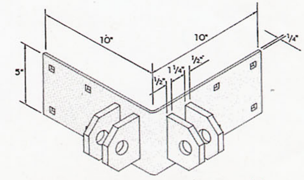
Corner T-Hinge Plate 4 Tab (Female) 6H410
