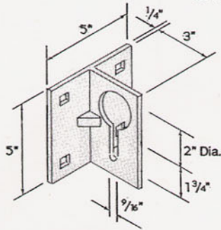
H.D. Key Hole Chain Holder 6H416
