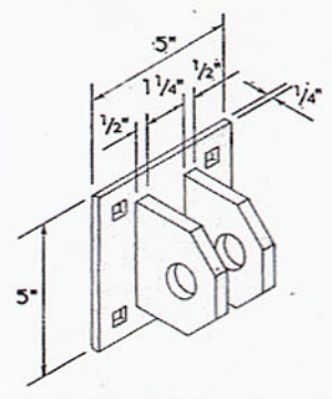
T-Hinge Plate 2 Tab (Female) 6H405
