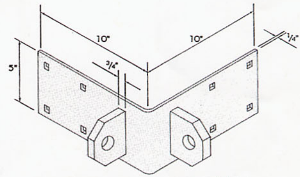
Corner T-Hinge Plate 2 Tab (Male) 6H408T
