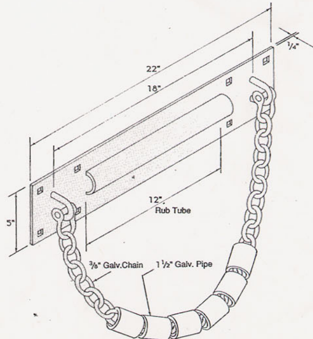
Pile Chain & Rub Plate Kit 9H421
