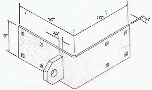
Corner Hinge Plate 1 Tab (Male) 6H407
