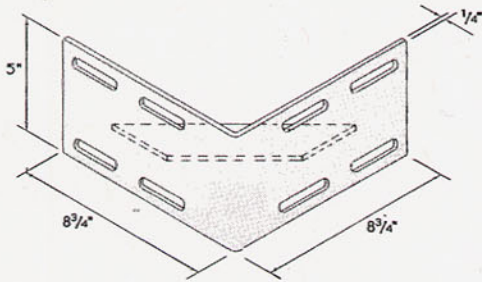
Inside Corner Plate 6H411
