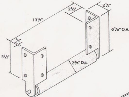
H.D. Key Hole Chain Holder 6H416
